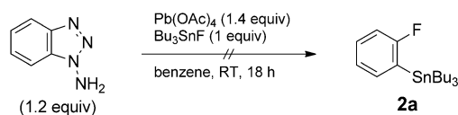
Scheme 4. Reaction of Bu 3 SnF with benzyne generated by oxidation.
